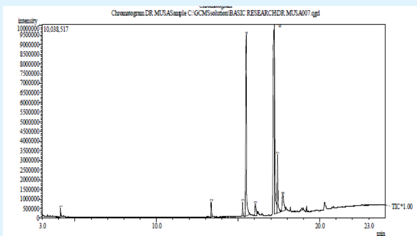
Figure 1: GC-MS Chromatogram of FAME of cottonseed. Figure one presented the GC/MS chromatograph of fatty acid methyl ester.
